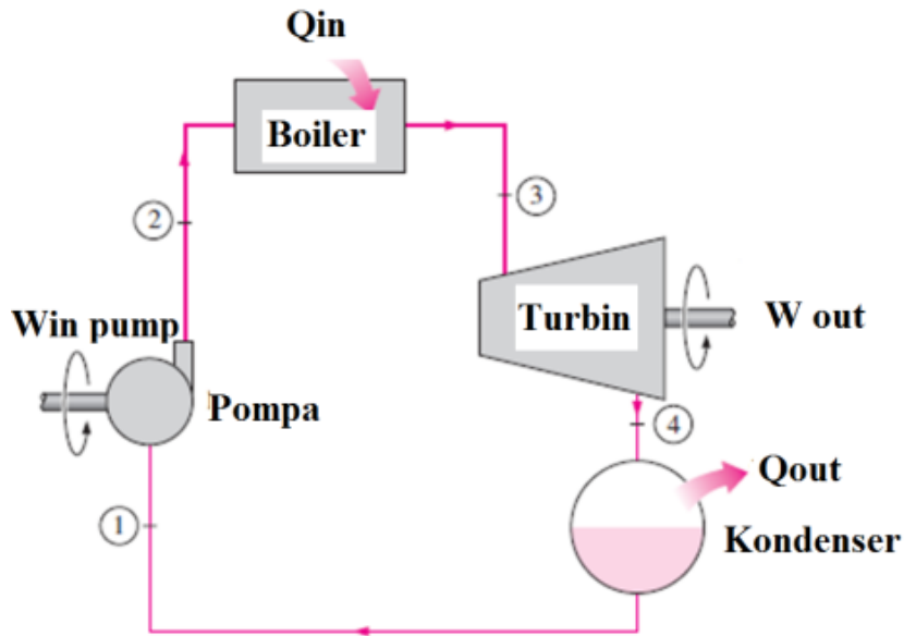
Gambar 4. Siklus Rankine [14]
